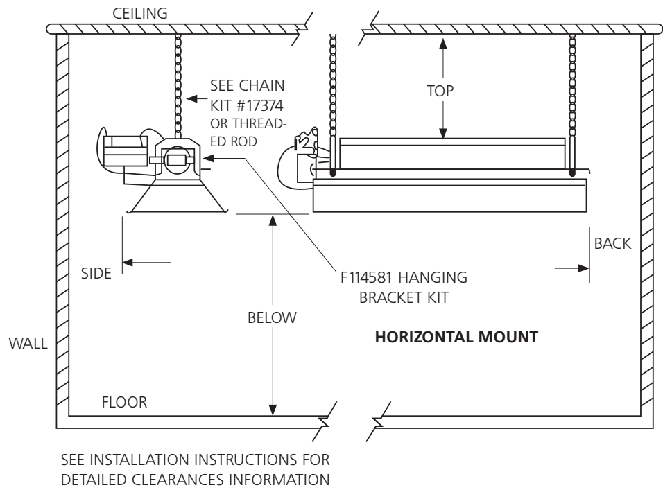
FIGURE 5 MOUNTING
