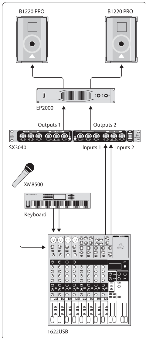
Fig. 3.1: Use of the SX3040 with live sound systems
