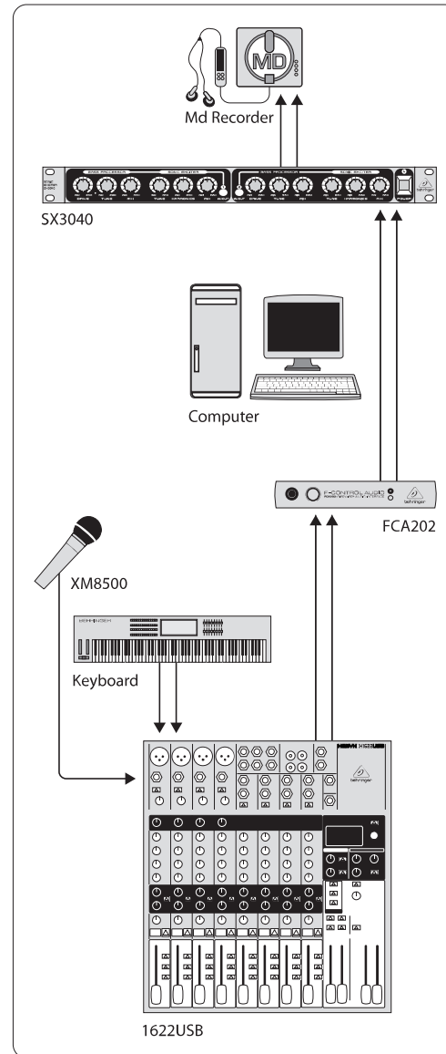
Fig. 3.2: The SX3040 in Studio mode
