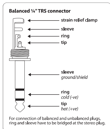
Fig. 4.2: Balanced jack cable with ¼" TRS jack plugs
