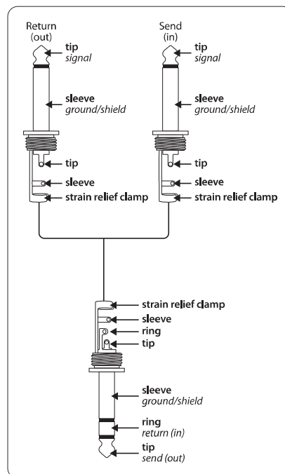
Fig. 4.4: Insert cable with one ¼" TRS (tip-ring-sleeve) jack plug on one end and two ¼" TS (tip-sleeve) jack plugs on the other end
