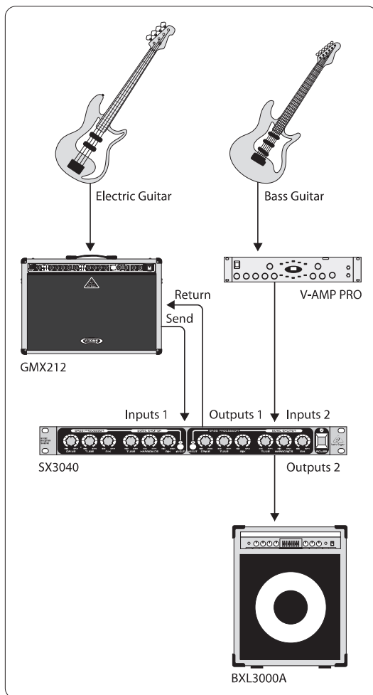
Fig. 3.3: The SX3040 in use with guitar amplifiers
