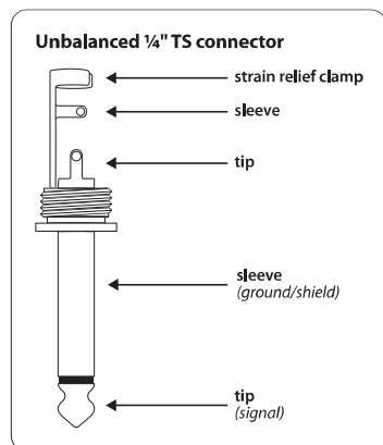
Fig. 4.1: Unbalanced jack cable with ¼" TS jack plugs
