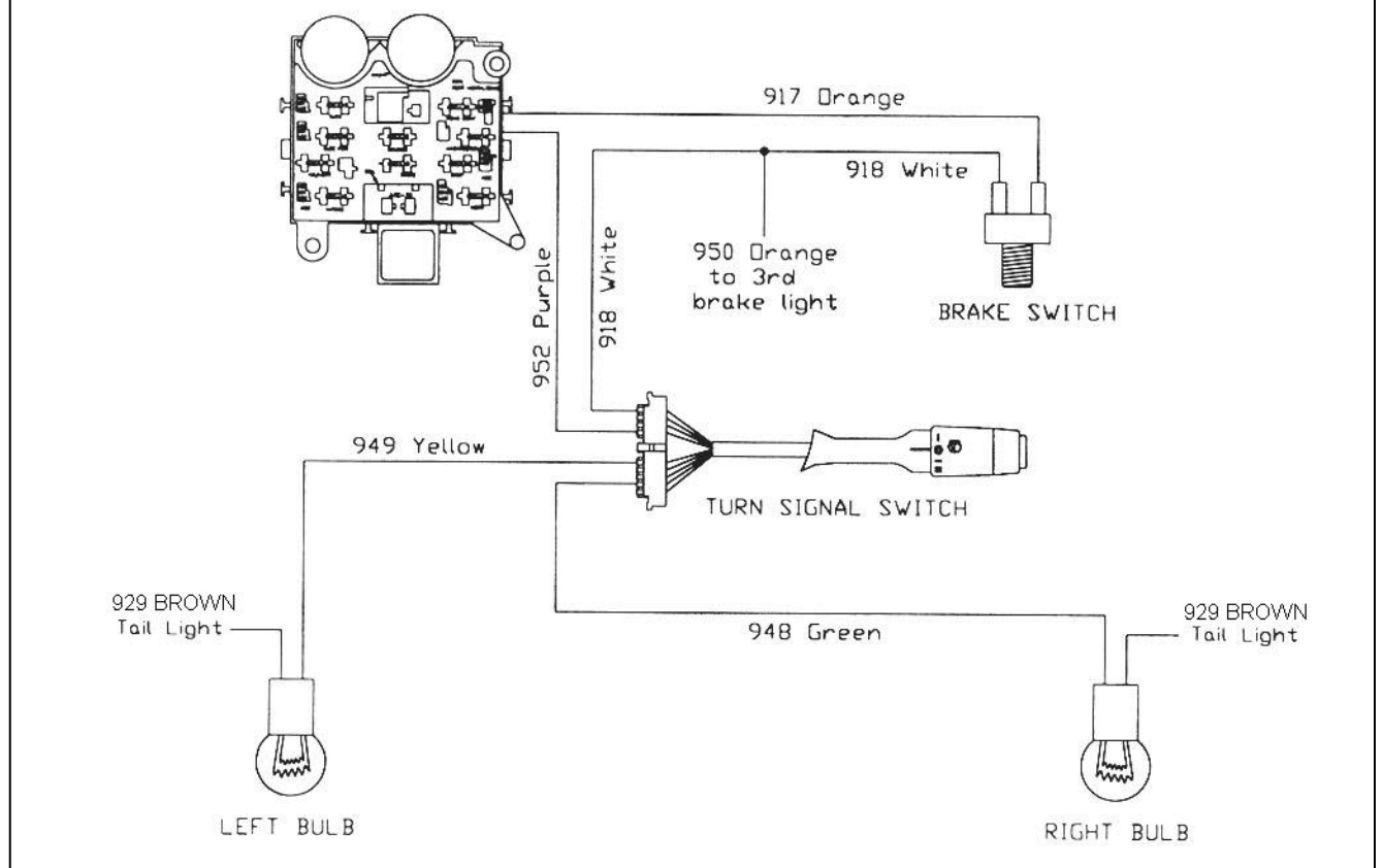
Figure 10-7A Integrated Brake Lights
