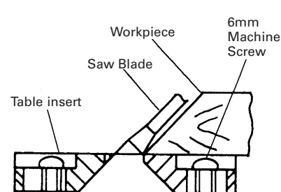
[Right bevel angle cutting] Fig. 9-c
