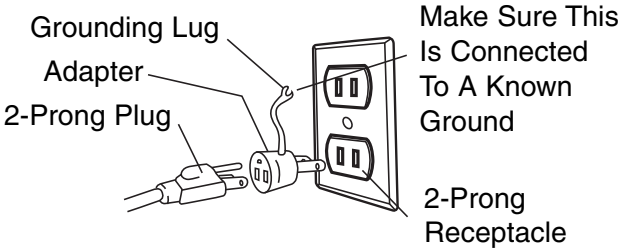
Figure 5 - 2-Prong Receptacle
